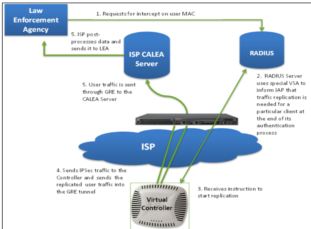
Figure 82 OAW-IAP to CALEA Server through VPN
