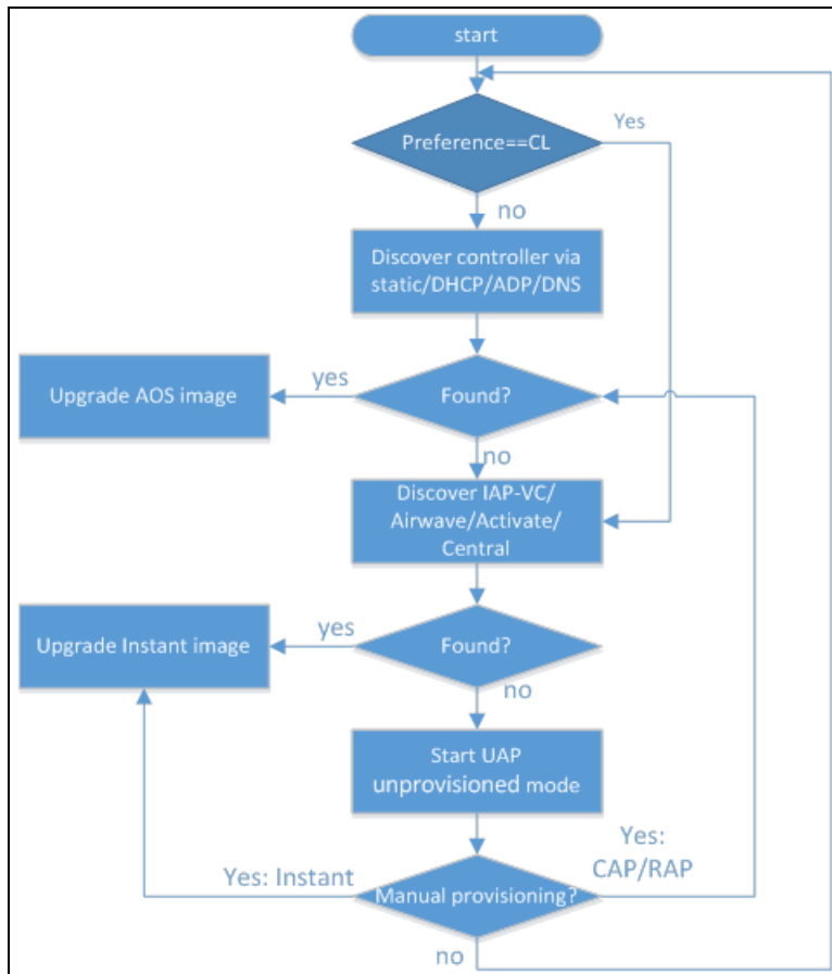
Figure 24 AP Discovery Logic
